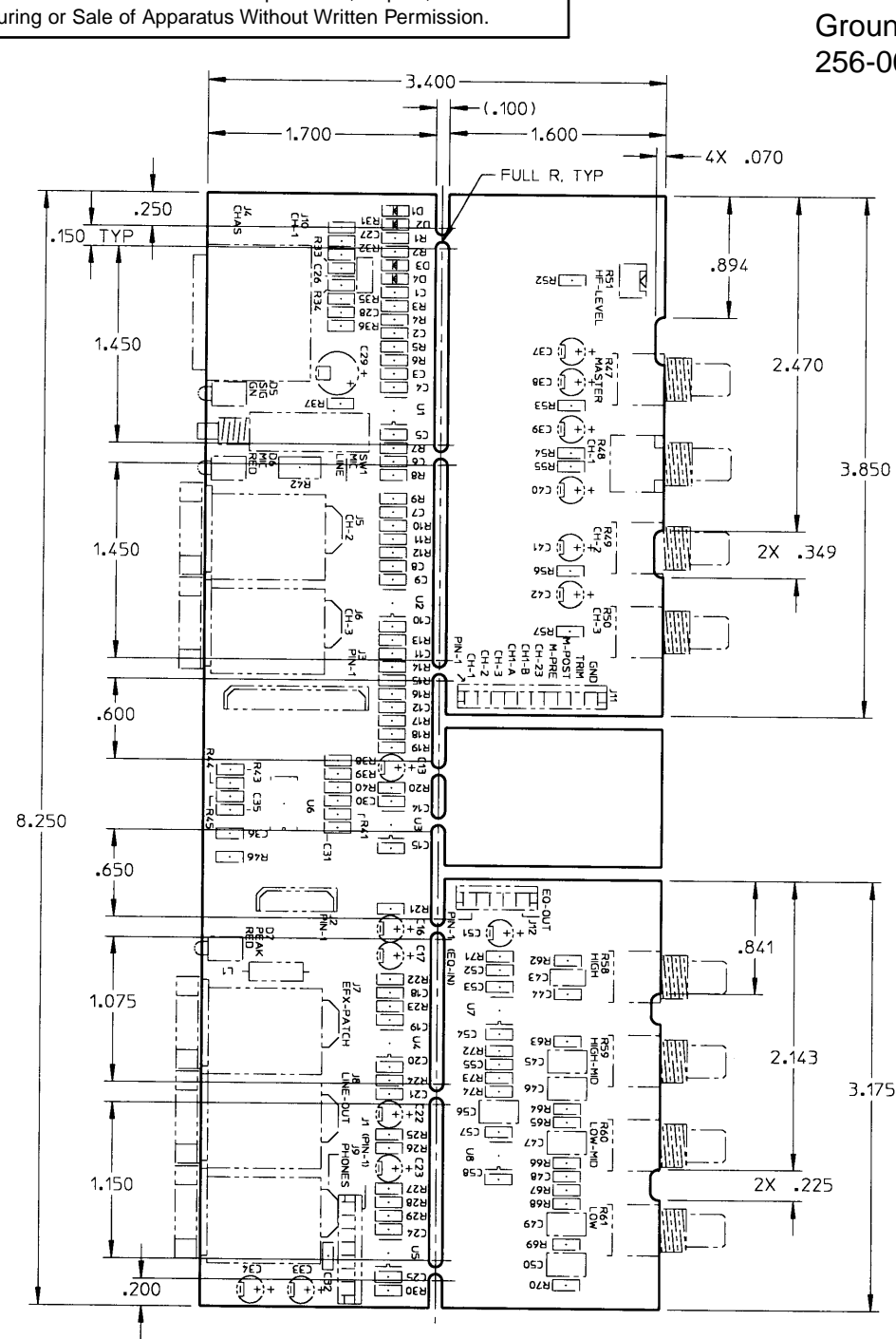
PCB Layout 510-00021-02
