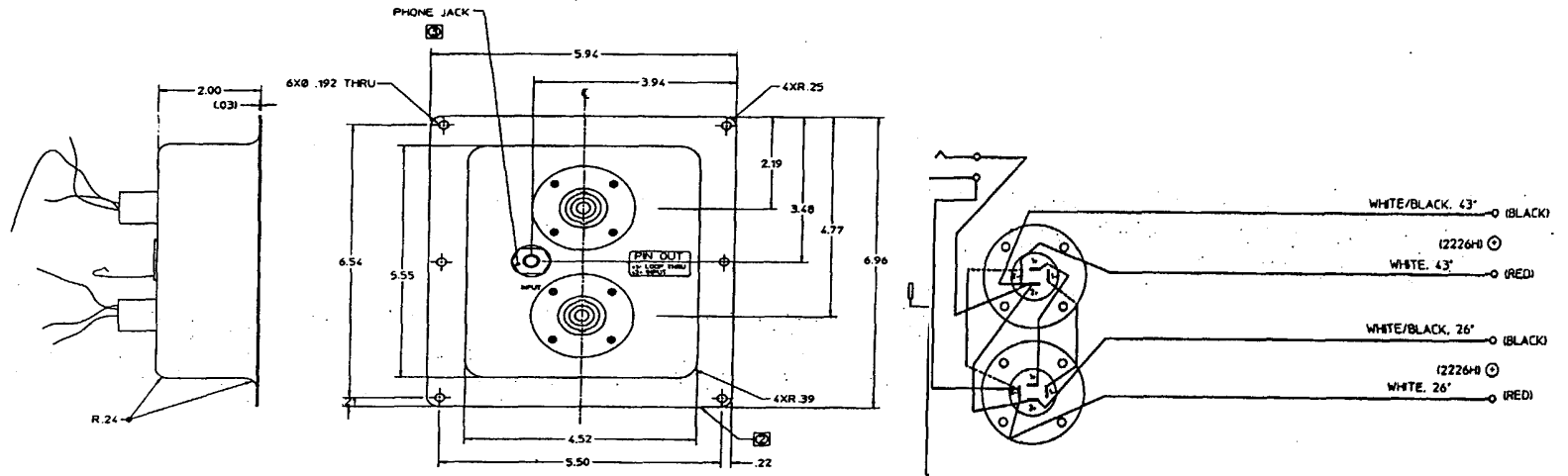
WIRING DIAGRAM OF 4-PIN NEUTRICK CONNECTOR (DL4MPRI)
